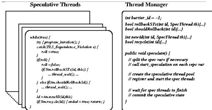
Fig. 5. The Interaction between the Speculative Threads and the Thread Manager
