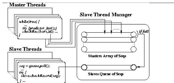
Fig. 6. “Inlining” - like Speculative Model. This figure presents the interaction between the Master/Slave Threads and the Slave Thread Manager
