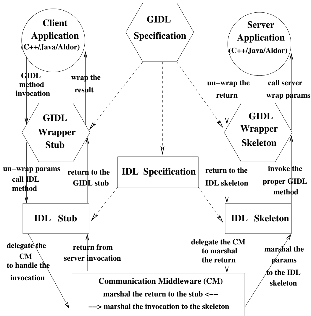
Fig. 4. GIDL architecture circle – user code; hexagon – GIDL component; rectangle – underlying architecture component; dashed arrow – is compiled to; solid arrow – method invocation flow
