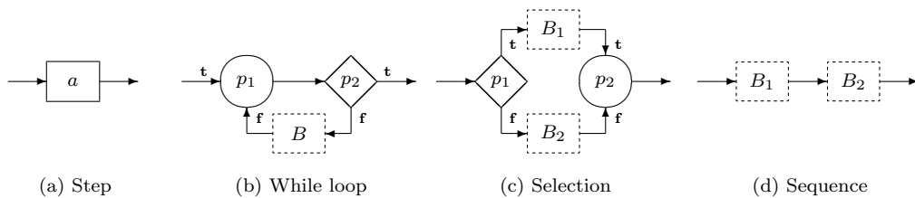
Fig. 1. Structured reversible flowcharts.
