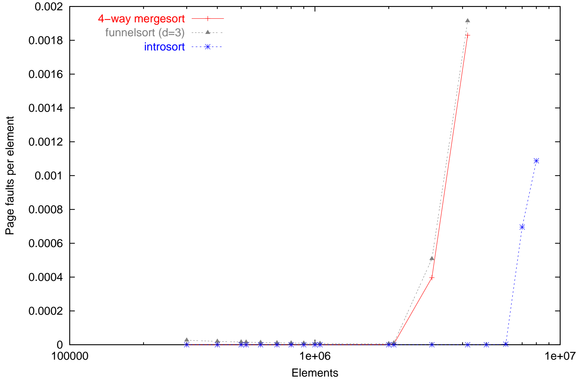
Page fault measurements of sorting on Pentium computer.
