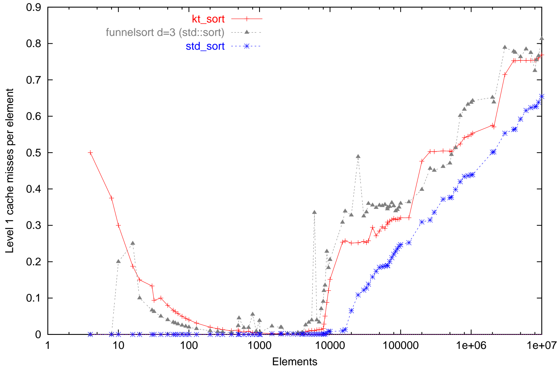
PAPI event count of sorting on Athlon computer.
