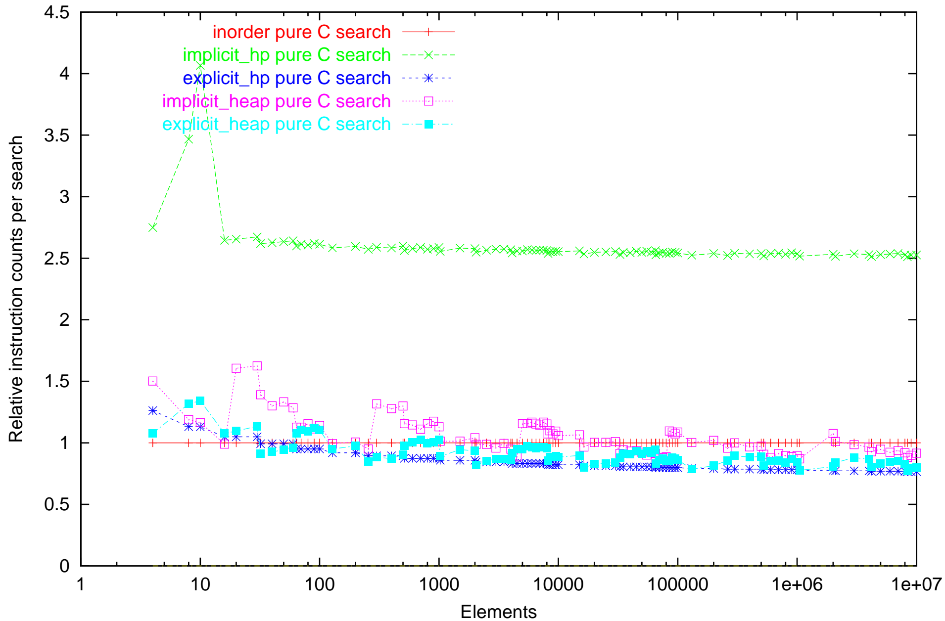
Instruction count of static search on Athlon computer. Dataset: unsuccessful
