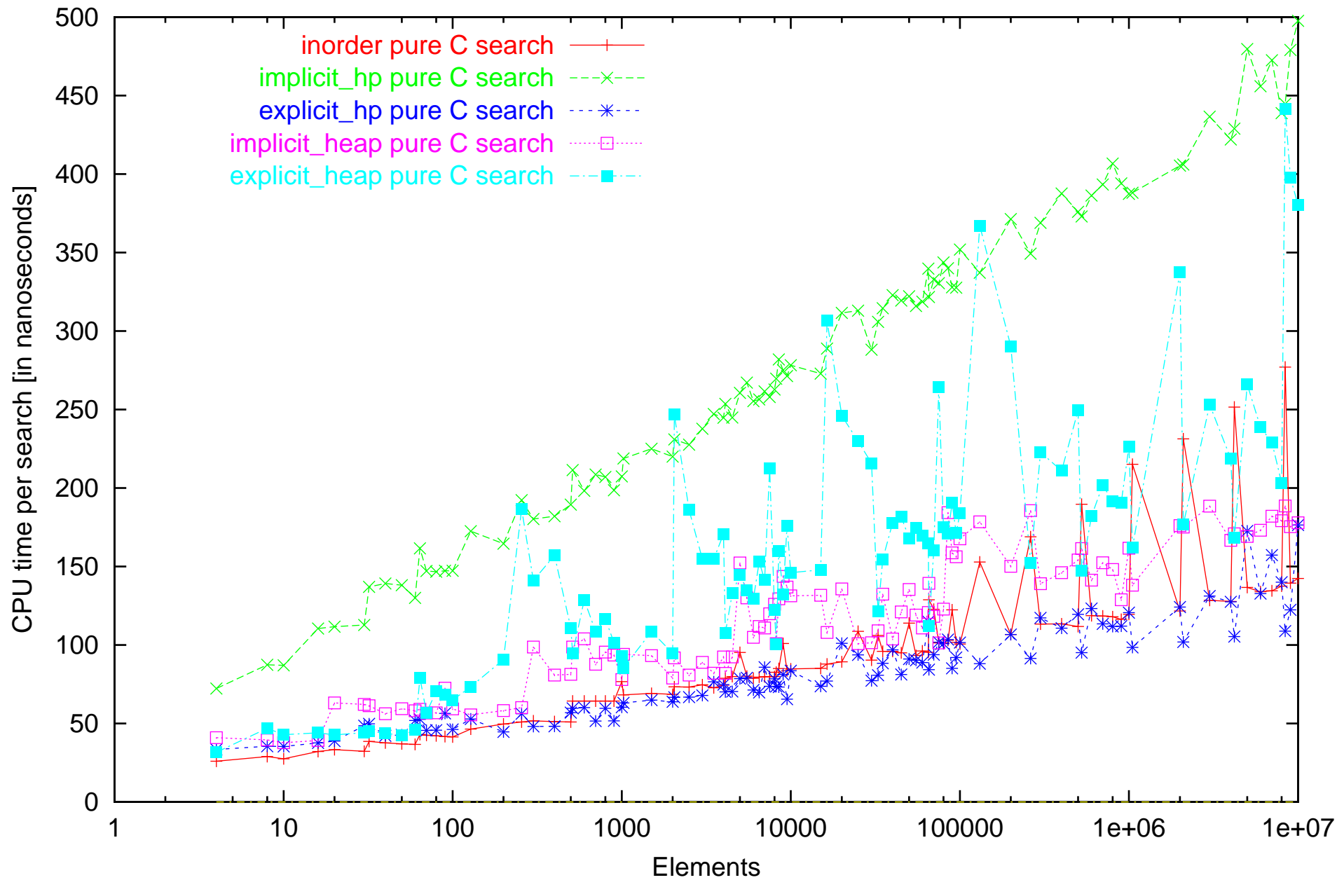
CPU time measurements of static search on Athlon computer. Dataset: unsuccessful
