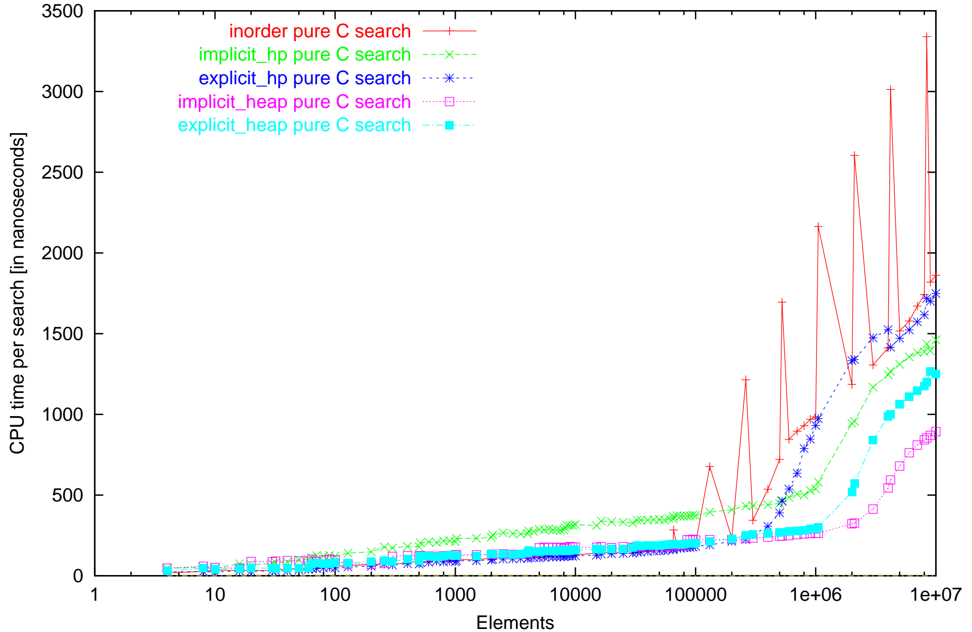
CPU time measurements of static search on Athlon computer. Dataset: successfull_repetitive_cycle
