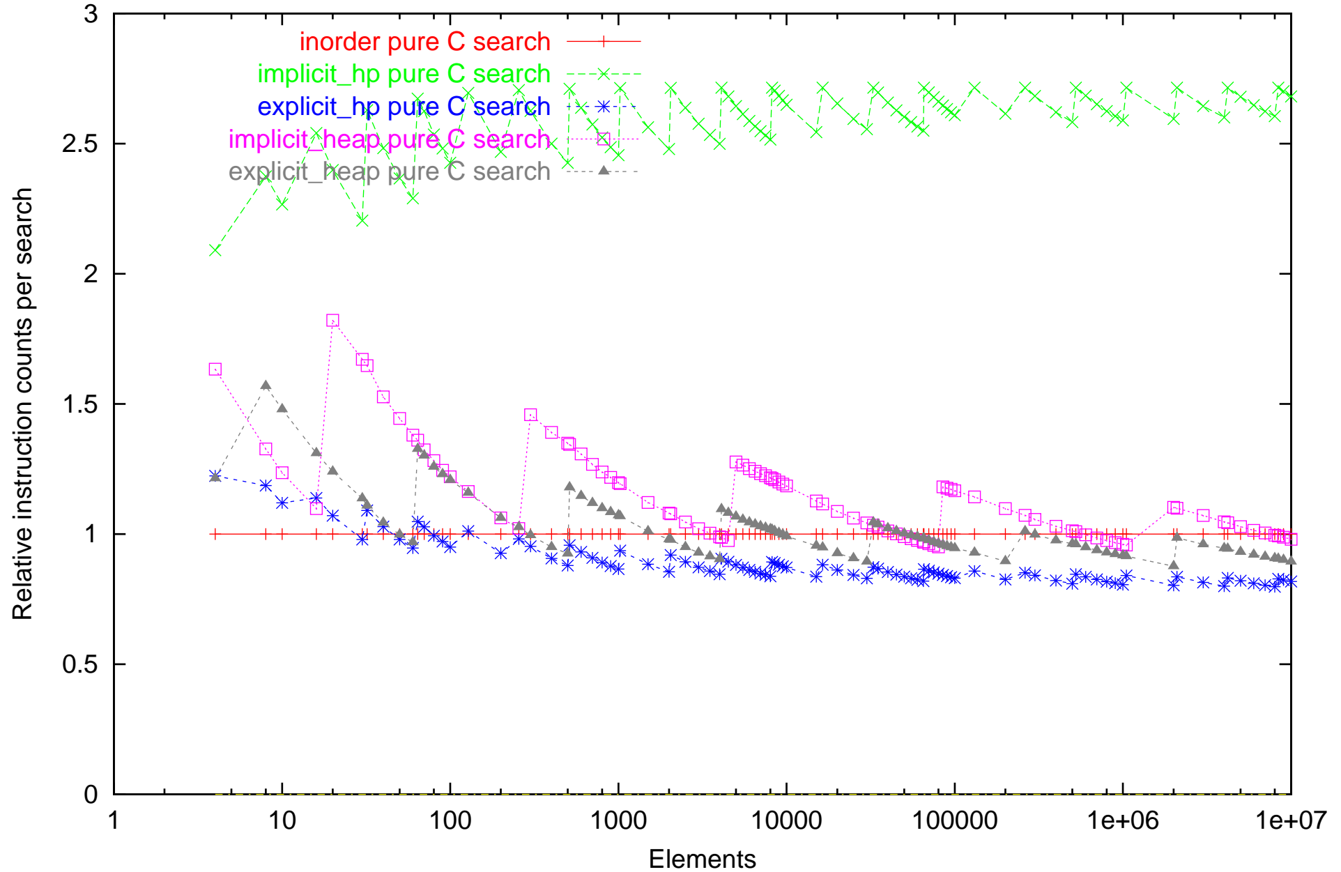
Instruction count of static search on Athlon computer. Dataset: successfull_random
