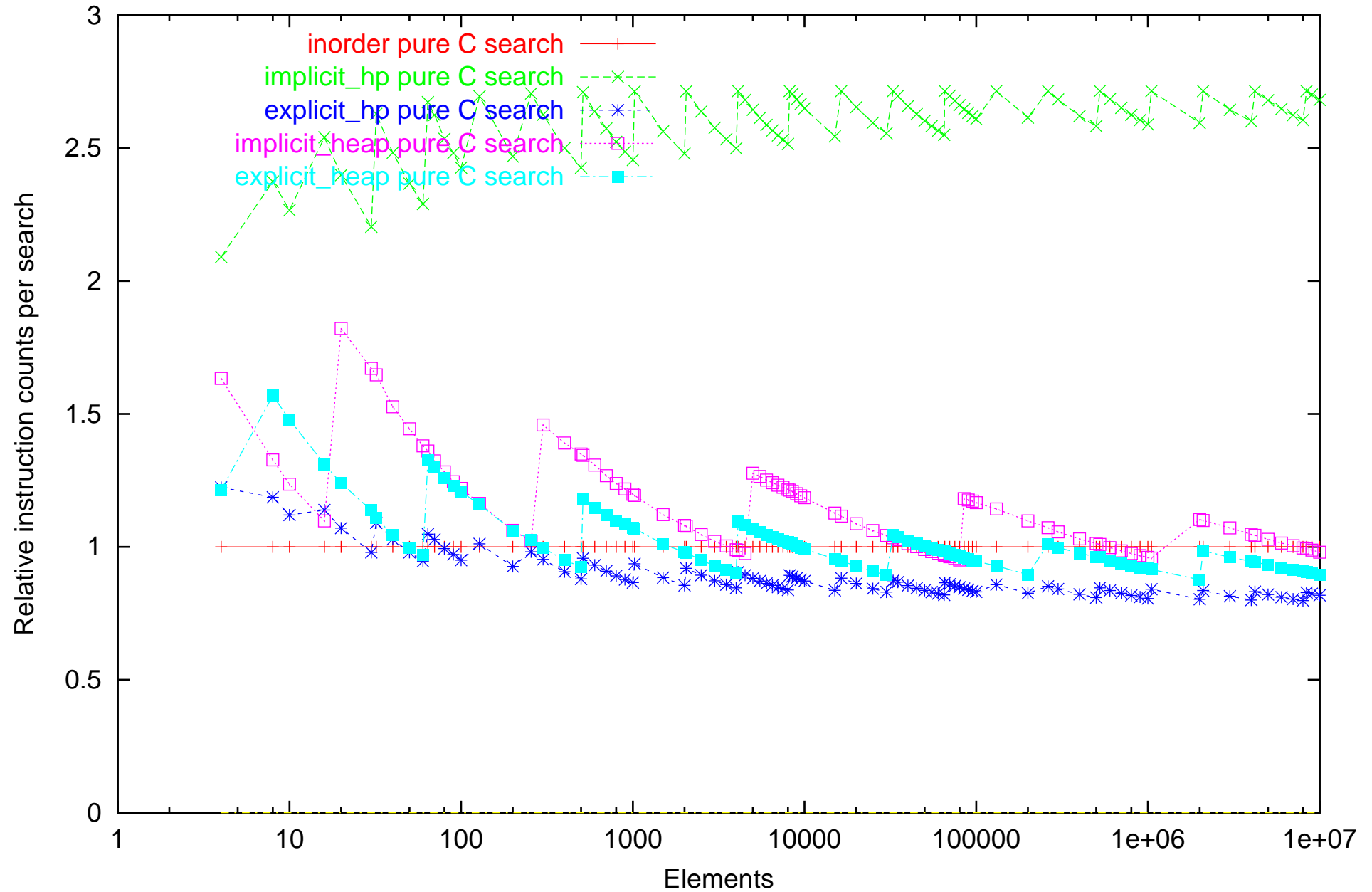
Instruction count of static search on Athlon computer. Dataset: successfull_increasing
