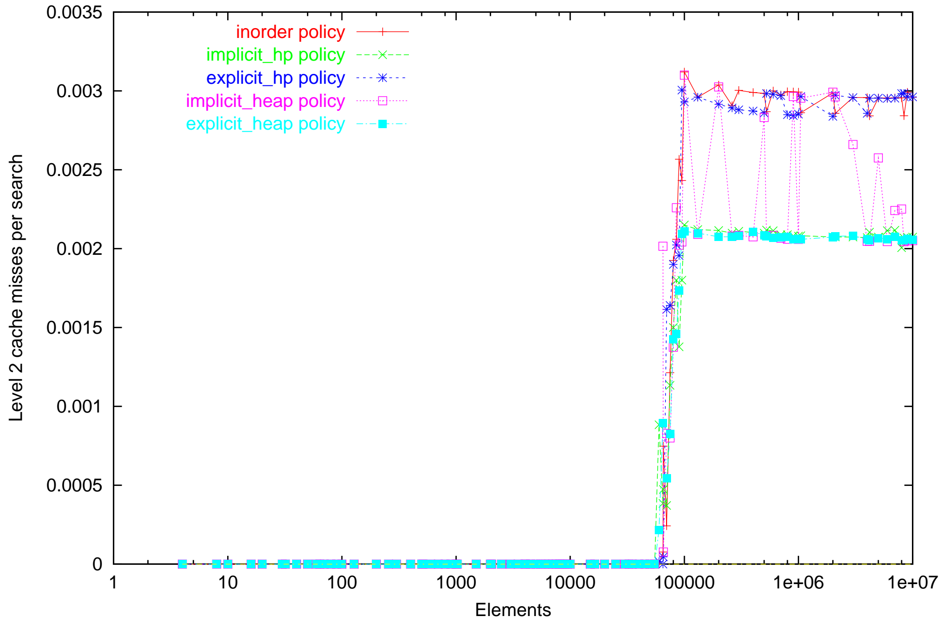
Level 2 cache misses of static search on Athlon computer. Dataset: unsuccessful
