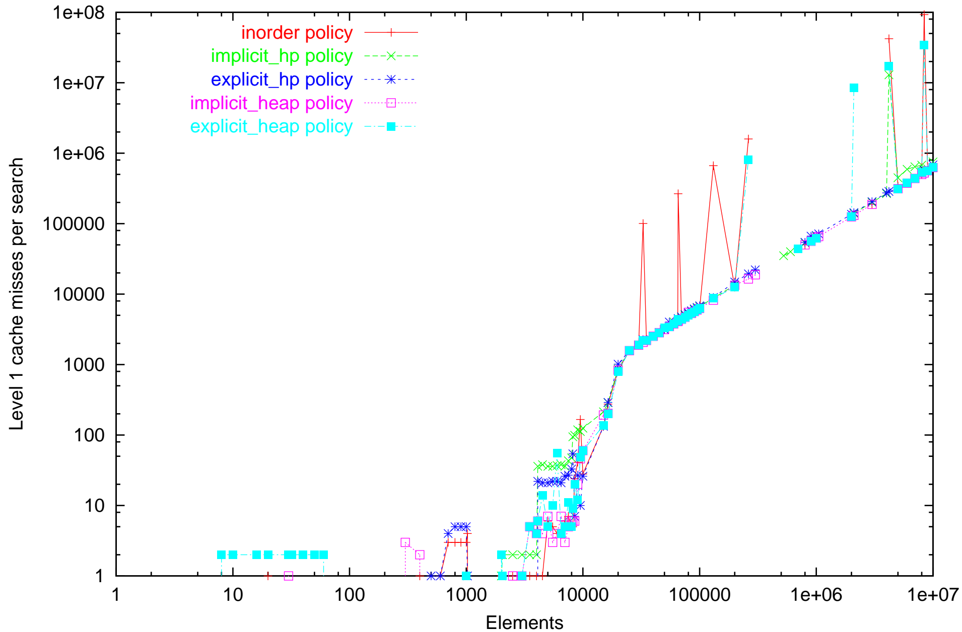
Level 1 cache misses of static search on Athlon computer. Dataset: unsuccessful
