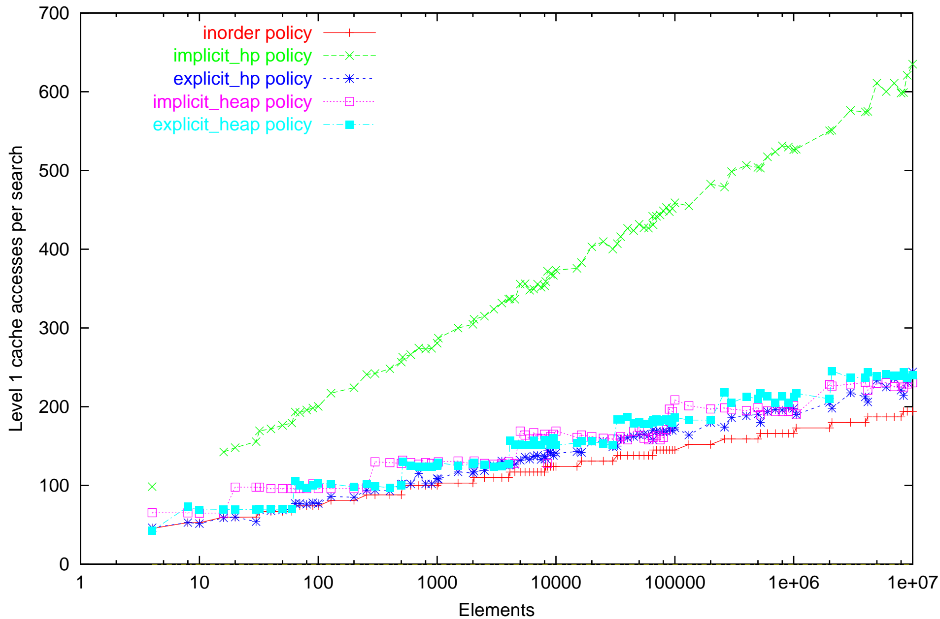
Level 1 cache accesses of static search on Athlon computer. Dataset: unsuccessful
