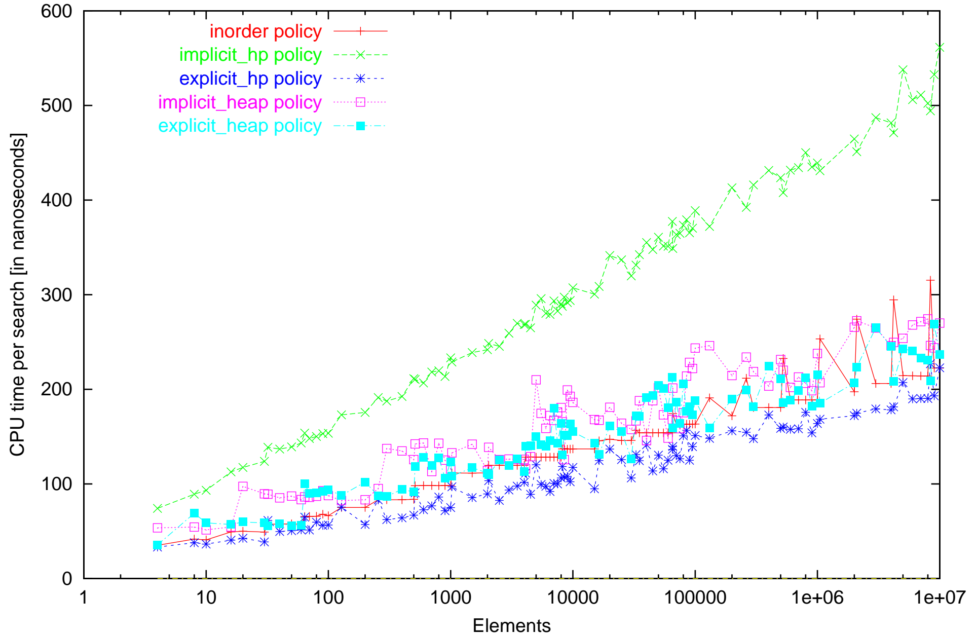
CPU time measurements of static search on Athlon computer. Dataset: unsuccessful
