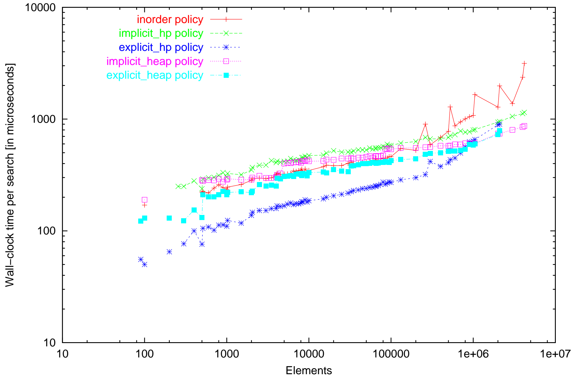
Wall clock time measurements of static search on Pentium computer. Dataset: successfull_repetitive_cycle
