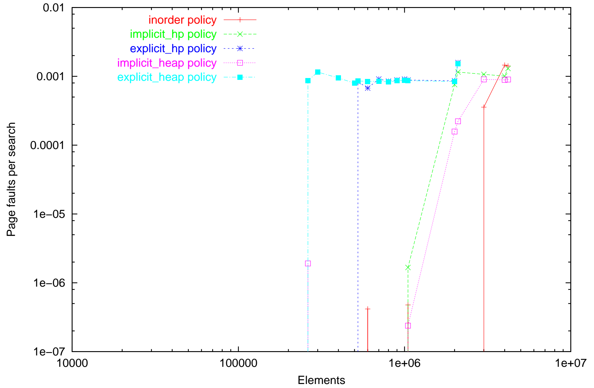
Page fault measurements of static search on Pentium computer. Dataset: successfull_repetitive_cycle
