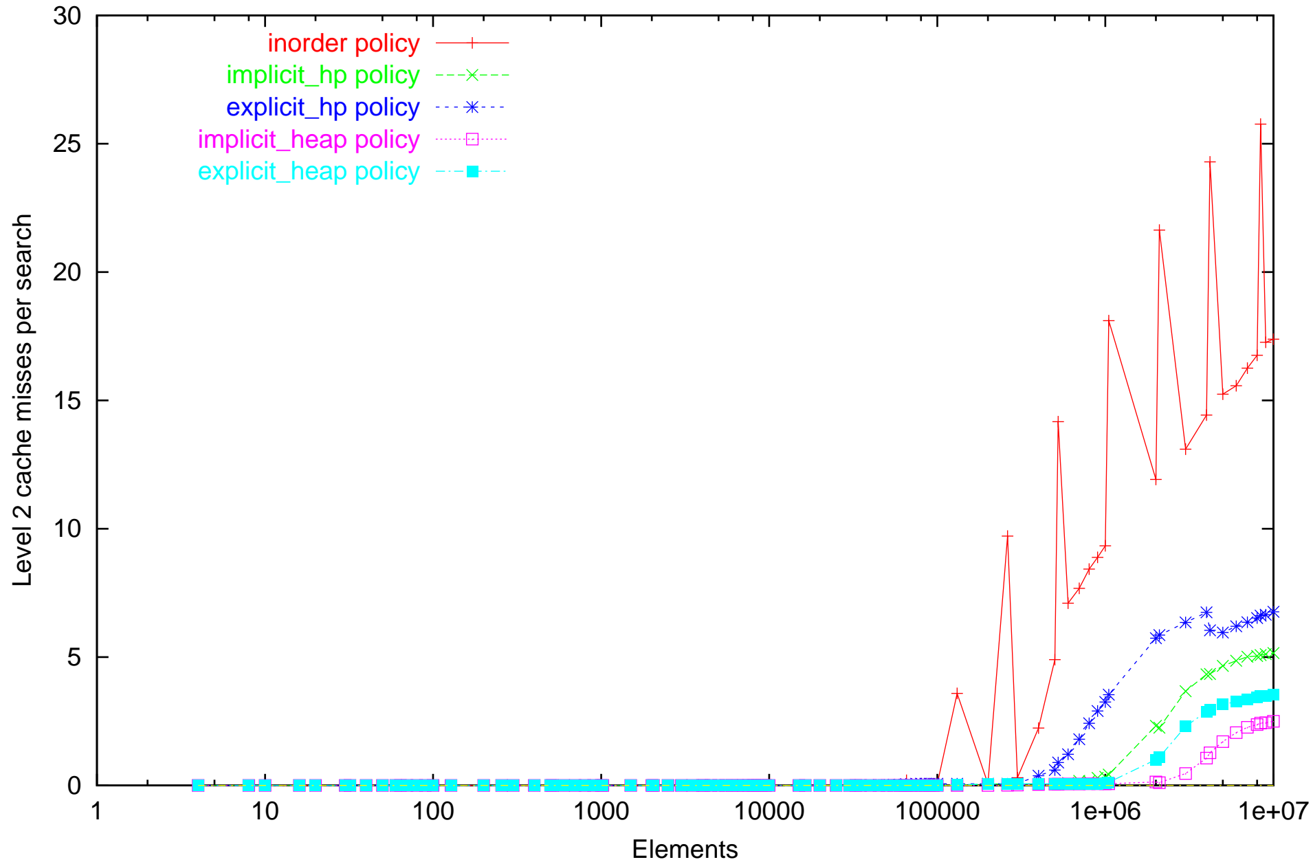
Level 2 cache misses of static search on Athlon computer. Dataset: successfull_repetitive_cycle
