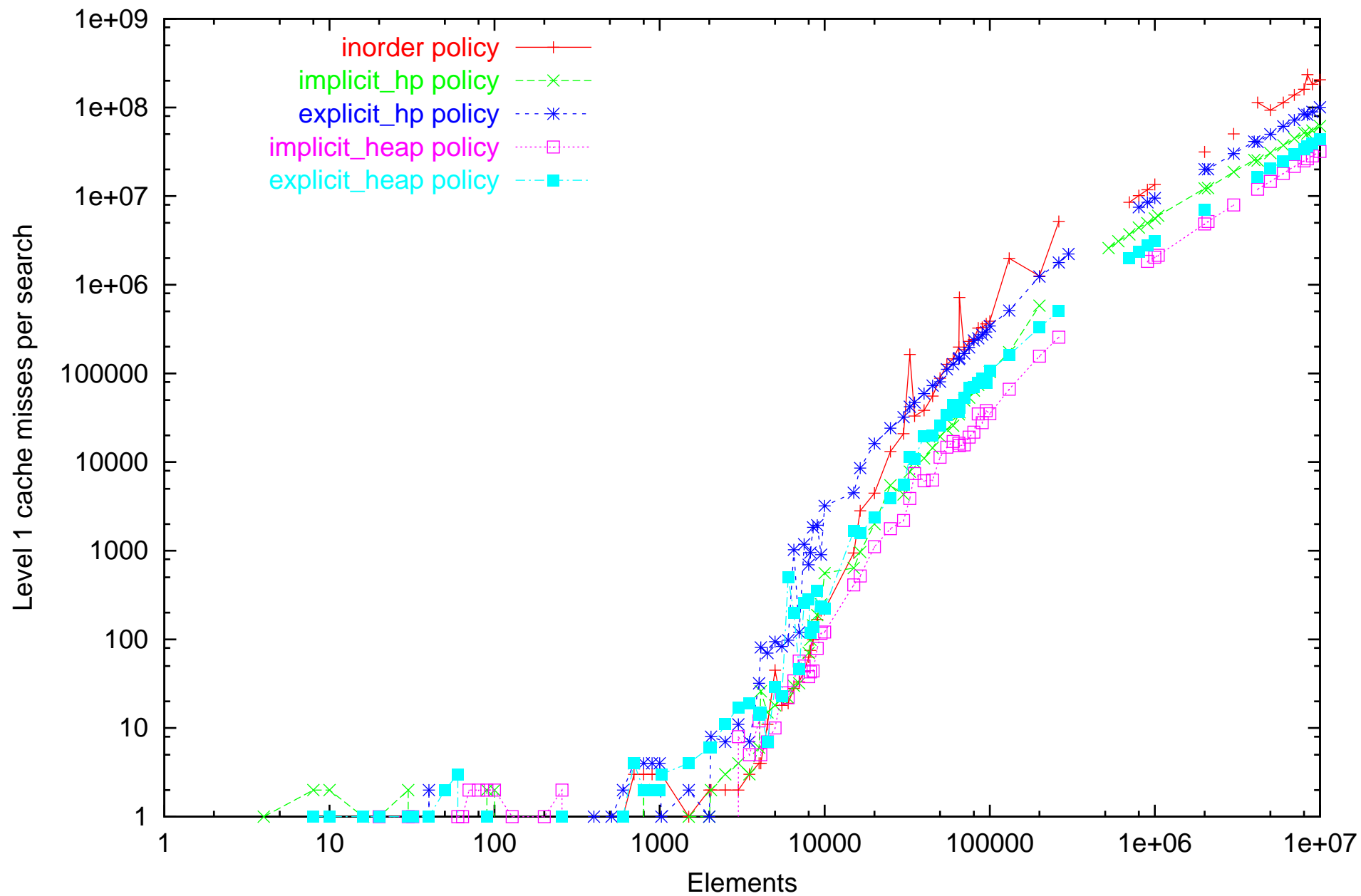
Level 1 cache misses of static search on Athlon computer. Dataset: successfull_repetitive_cycle
