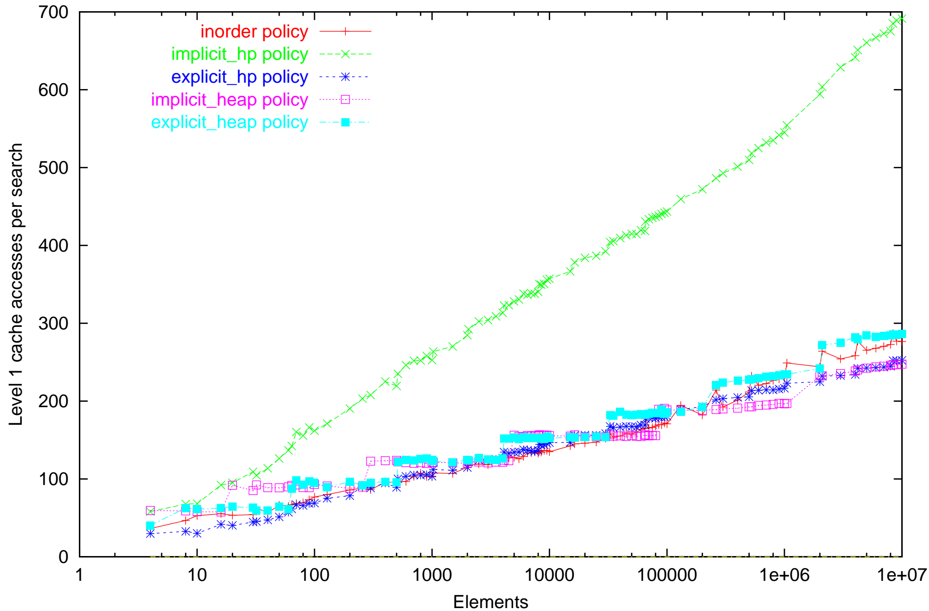
Level 1 cache accesses of static search on Athlon computer. Dataset: successfull_repetitive_cycle
