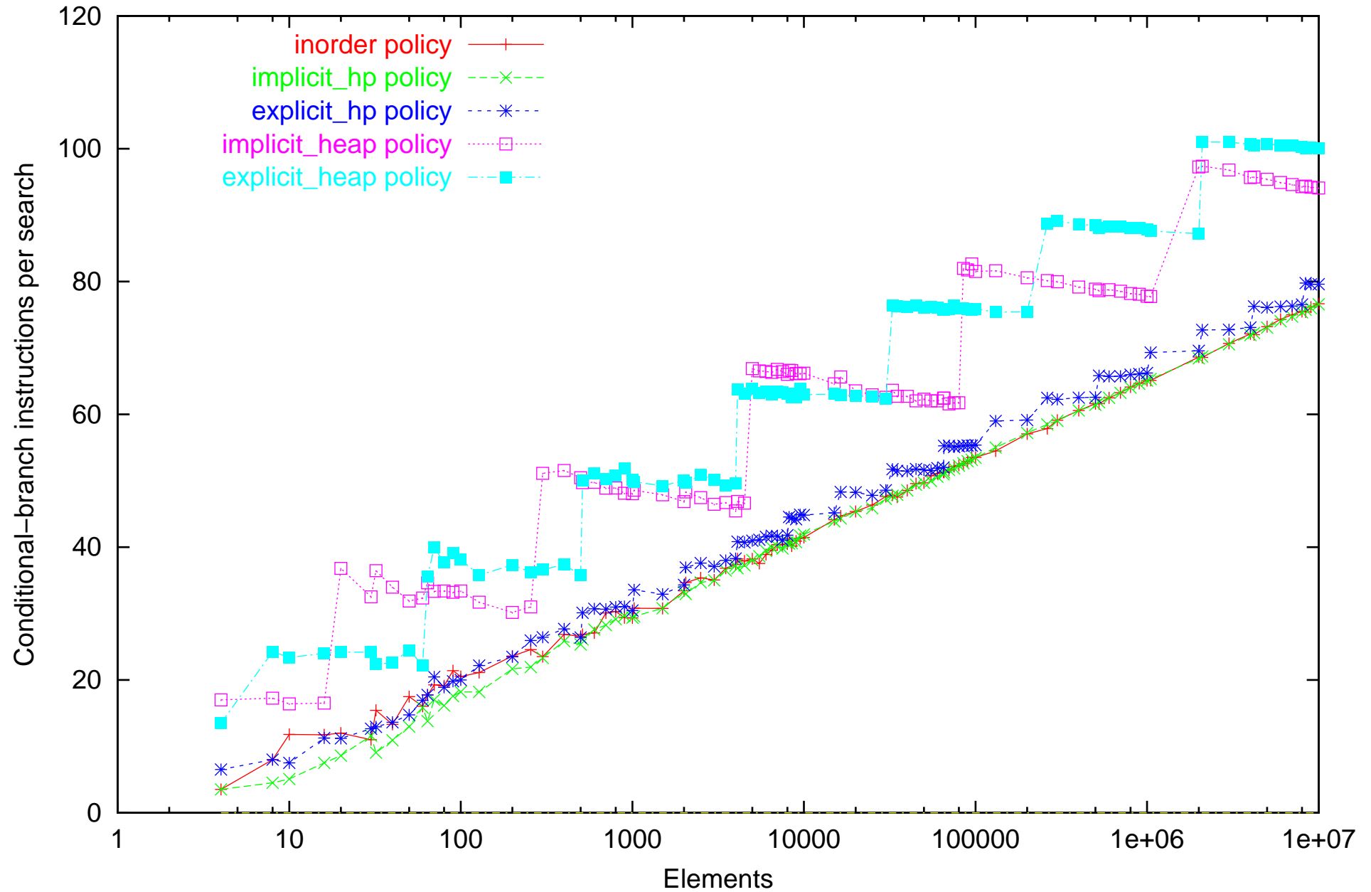
PAPI event count of static search on Athlon computer. Dataset: successfull_repetitive_cycle
