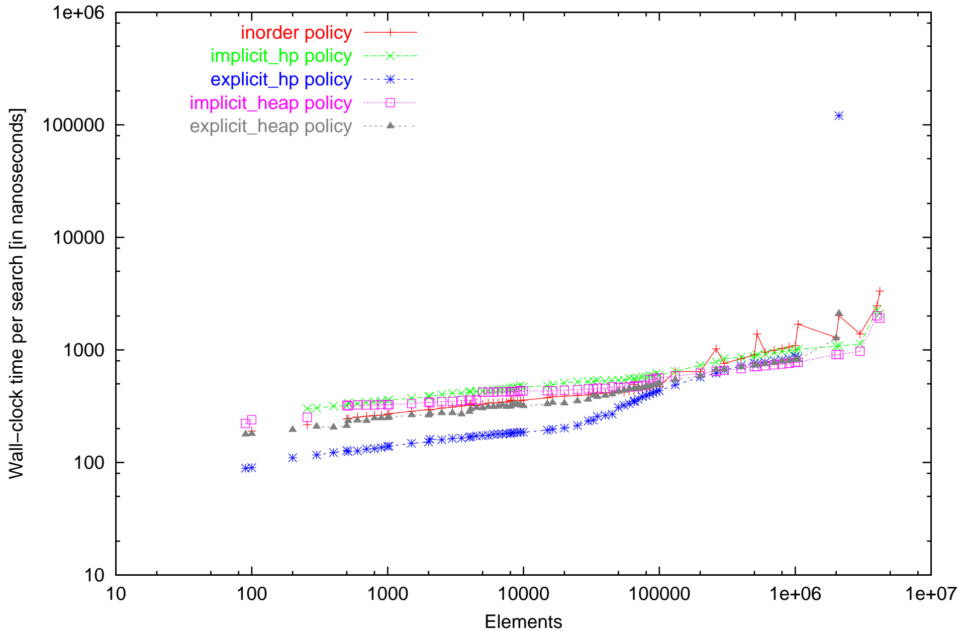
Wall clock time measurements of static search on Pentium computer. Dataset: successfull_random
