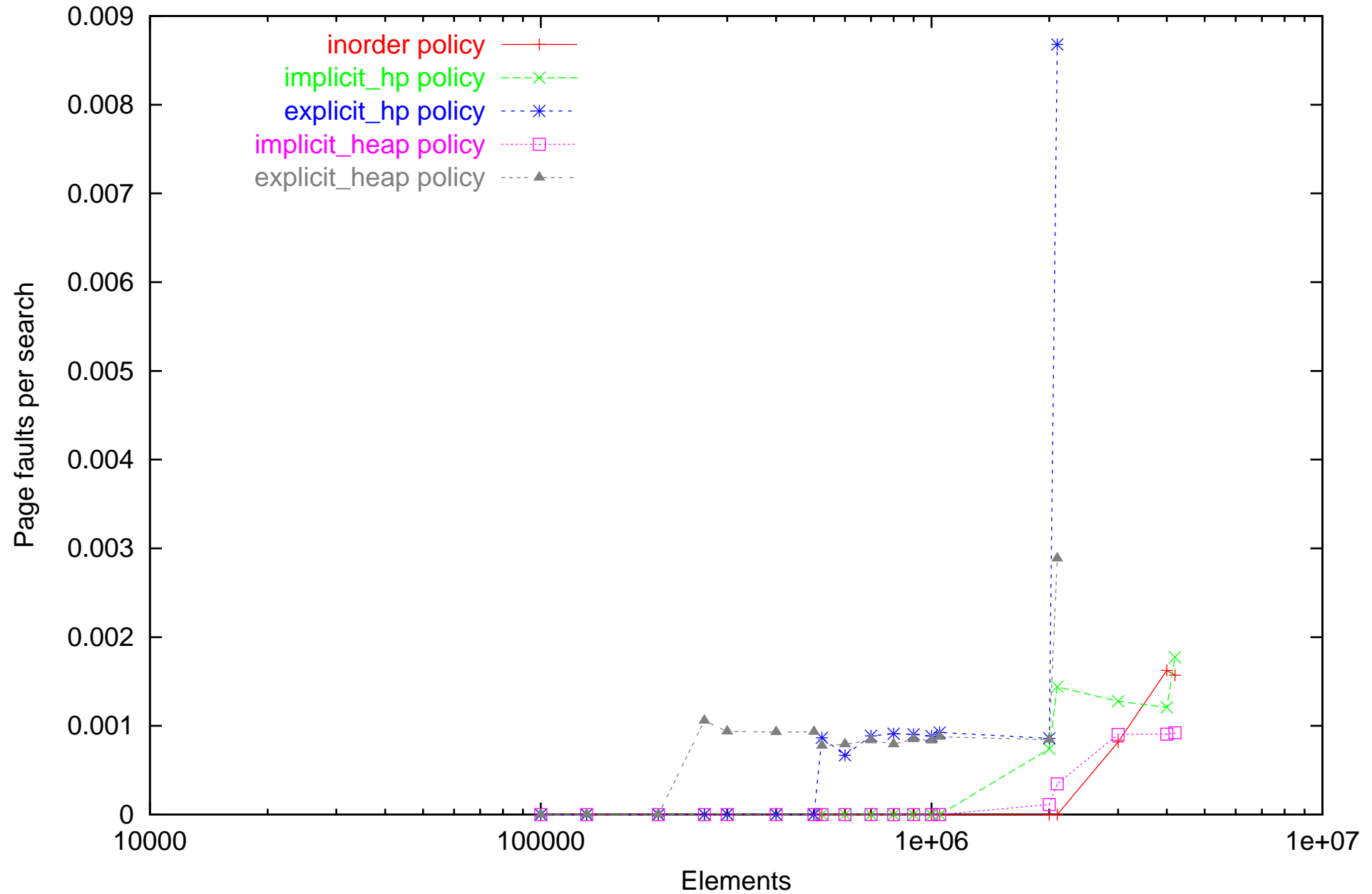
Page fault measurements of static search on Pentium computer. Dataset: successfull_random
