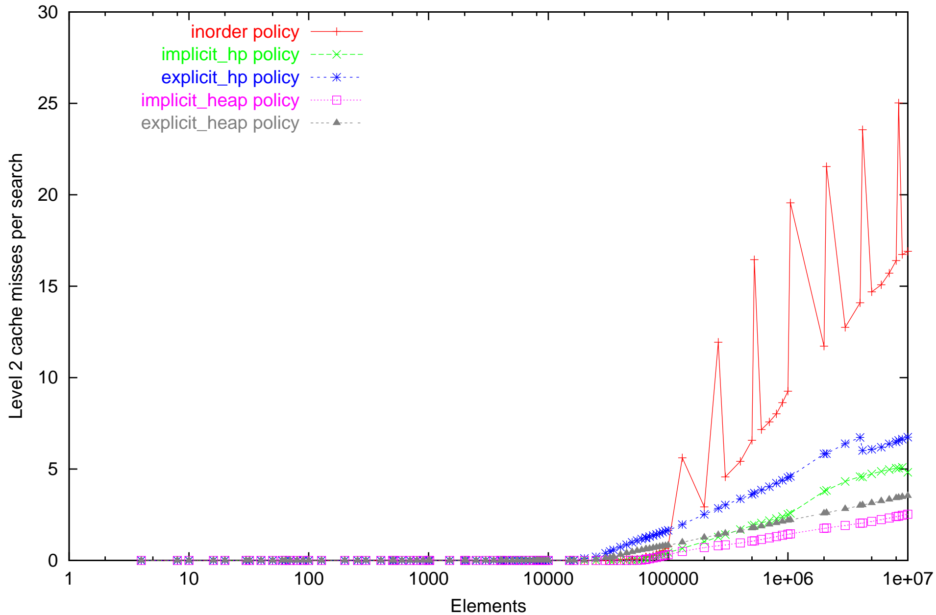
Level 2 cache misses of static search on Athlon computer. Dataset: successfull_random
