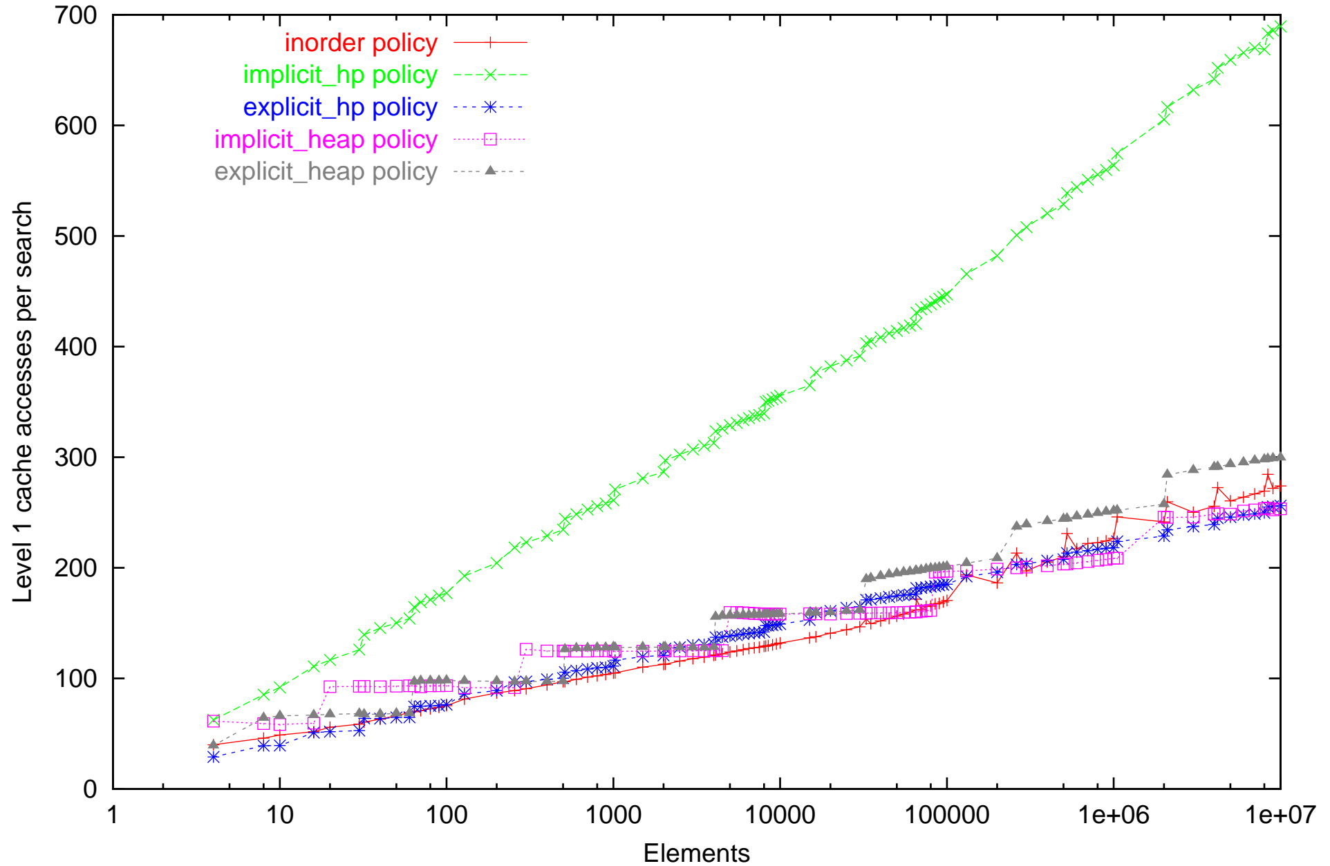
Level 1 cache accesses of static search on Athlon computer. Dataset: successfull_random
