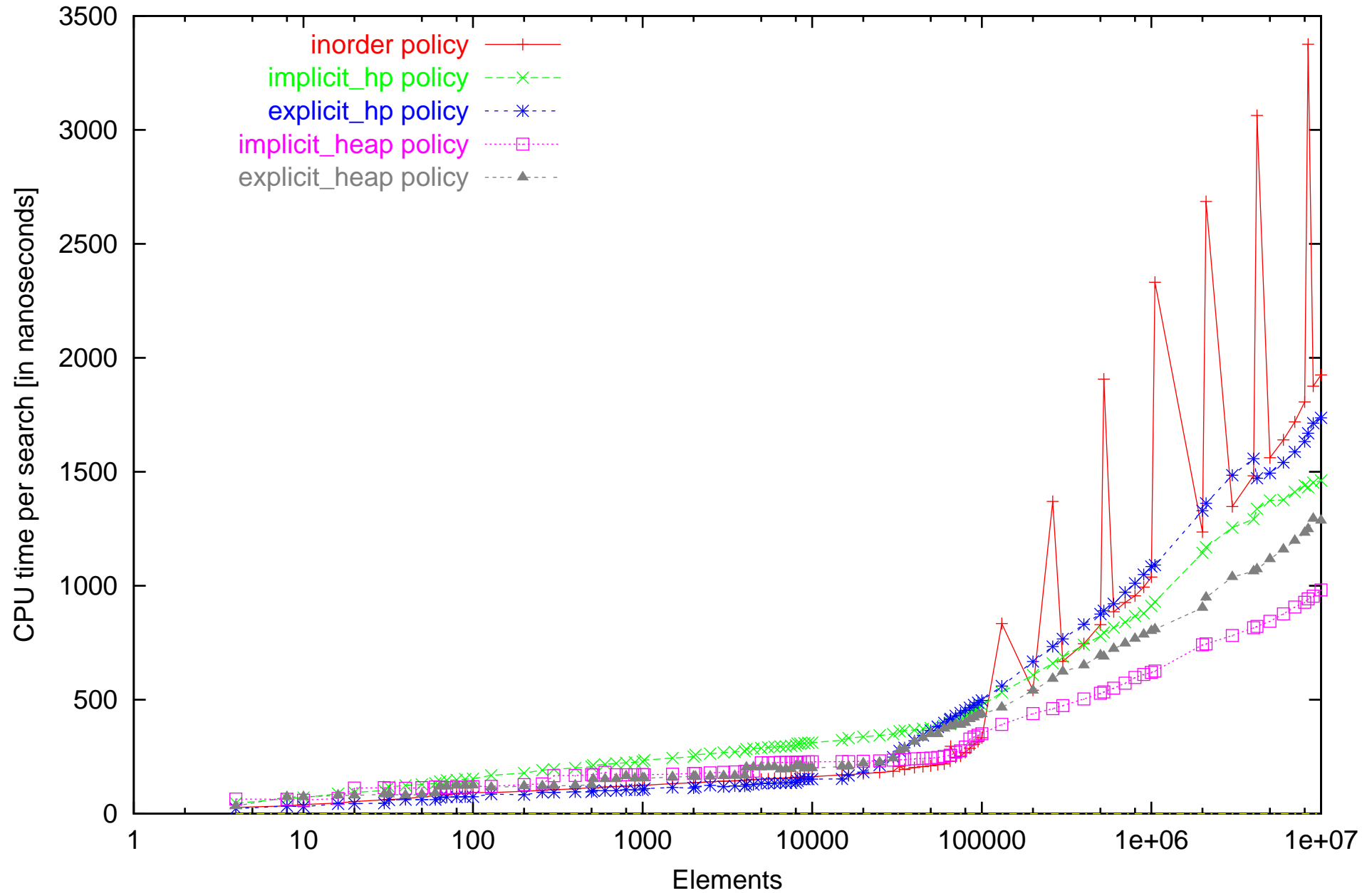
CPU time measurements of static search on Athlon computer. Dataset: successfull_random
