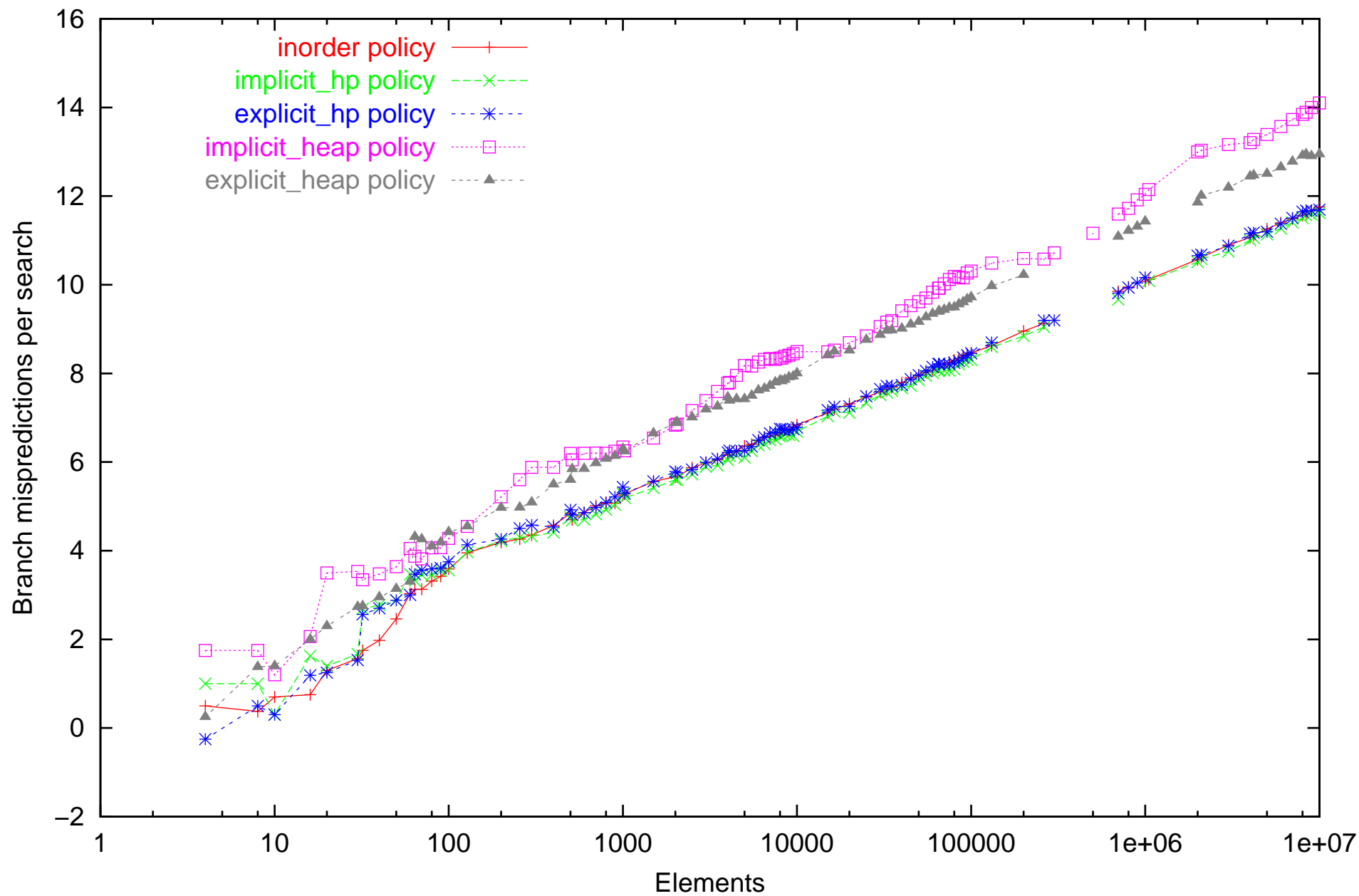
PAPI event count of static search on Athlon computer. Dataset: successfull_random
