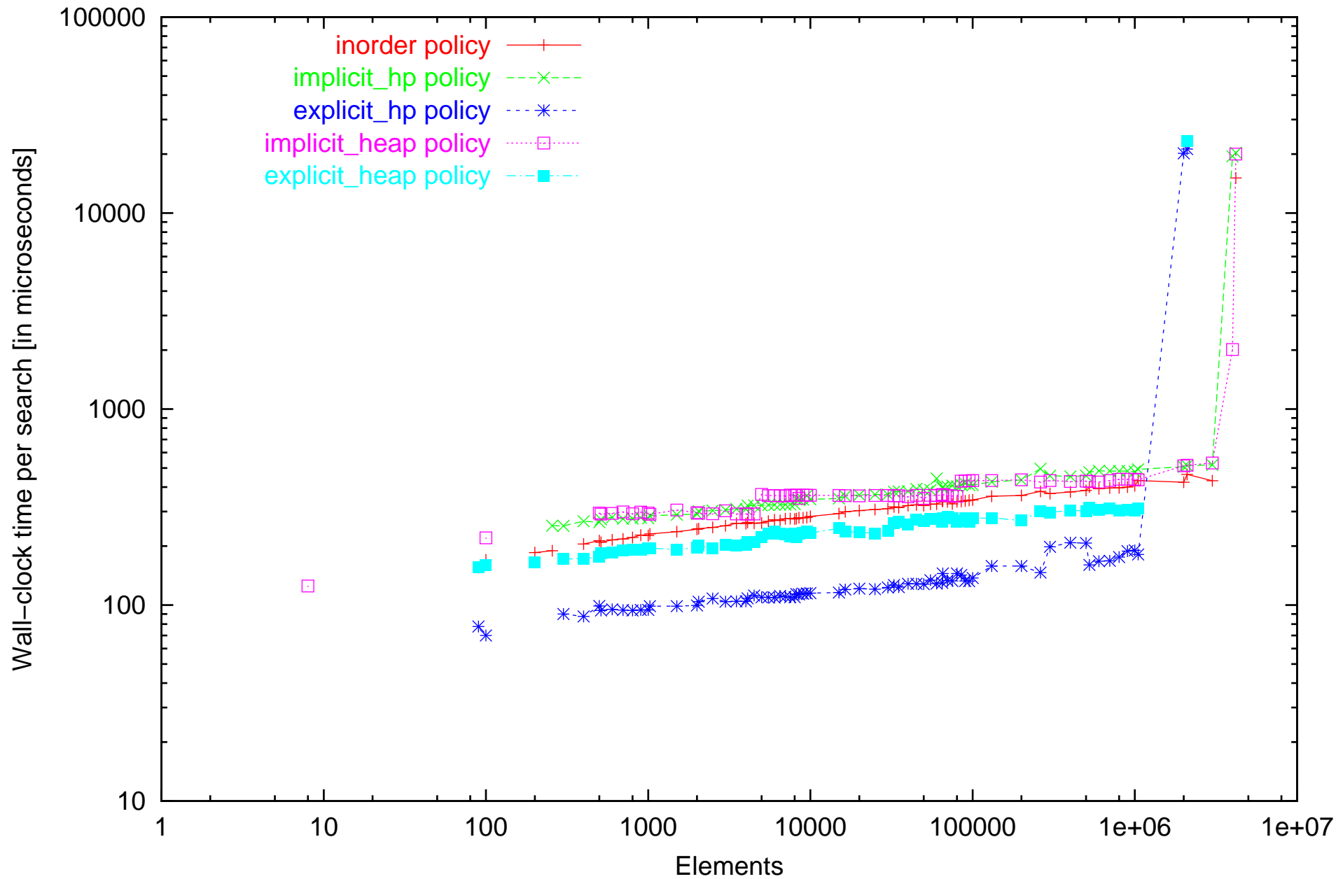
Wall clock time measurements of static search on Pentium computer. Dataset: successfull_increasing
