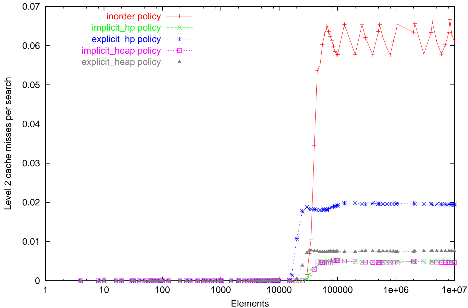
Level 2 cache misses of static search on Athlon computer. Dataset: successfull_increasing
