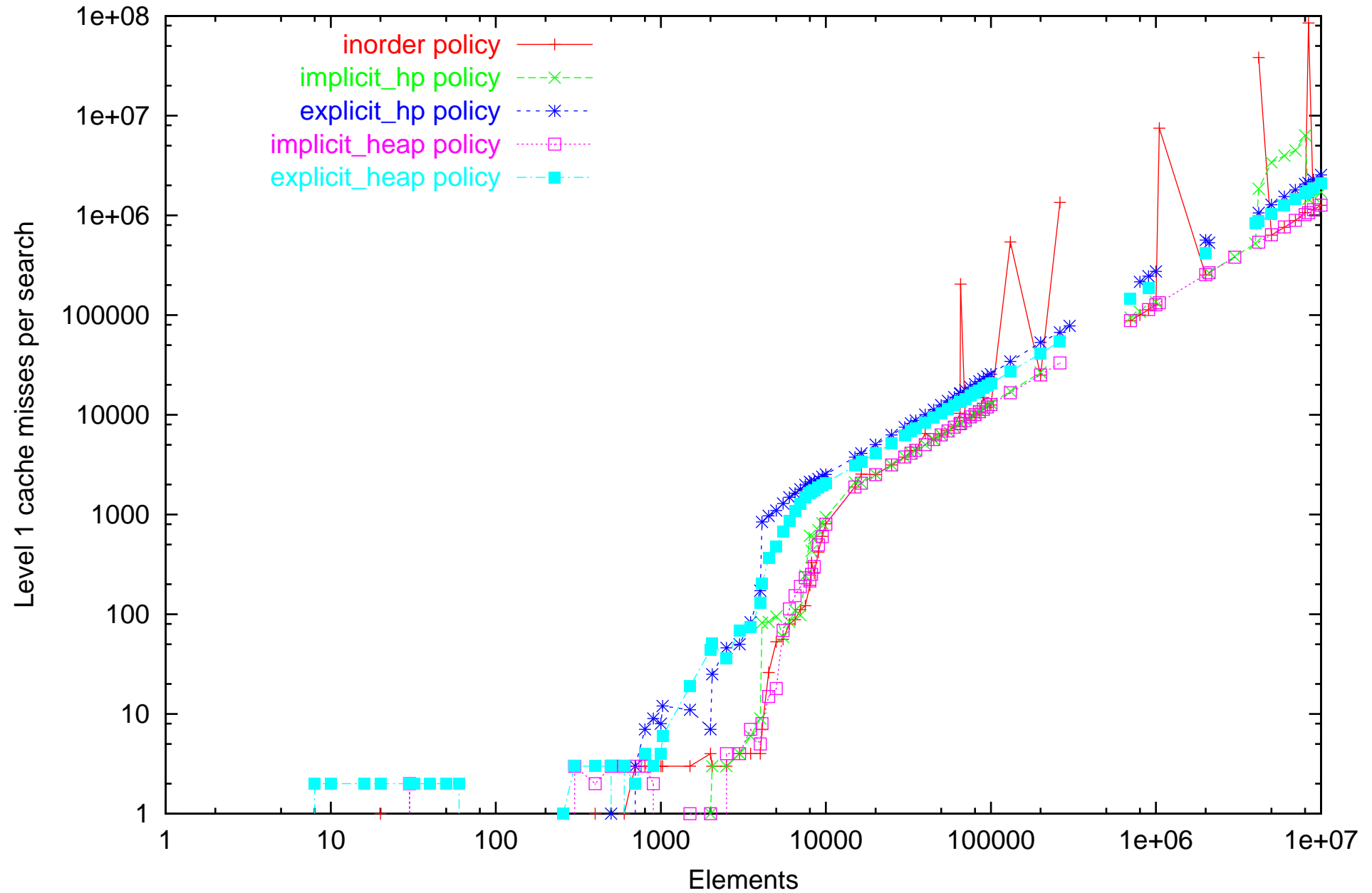
Level 1 cache misses of static search on Athlon computer. Dataset: successfull_increasing
