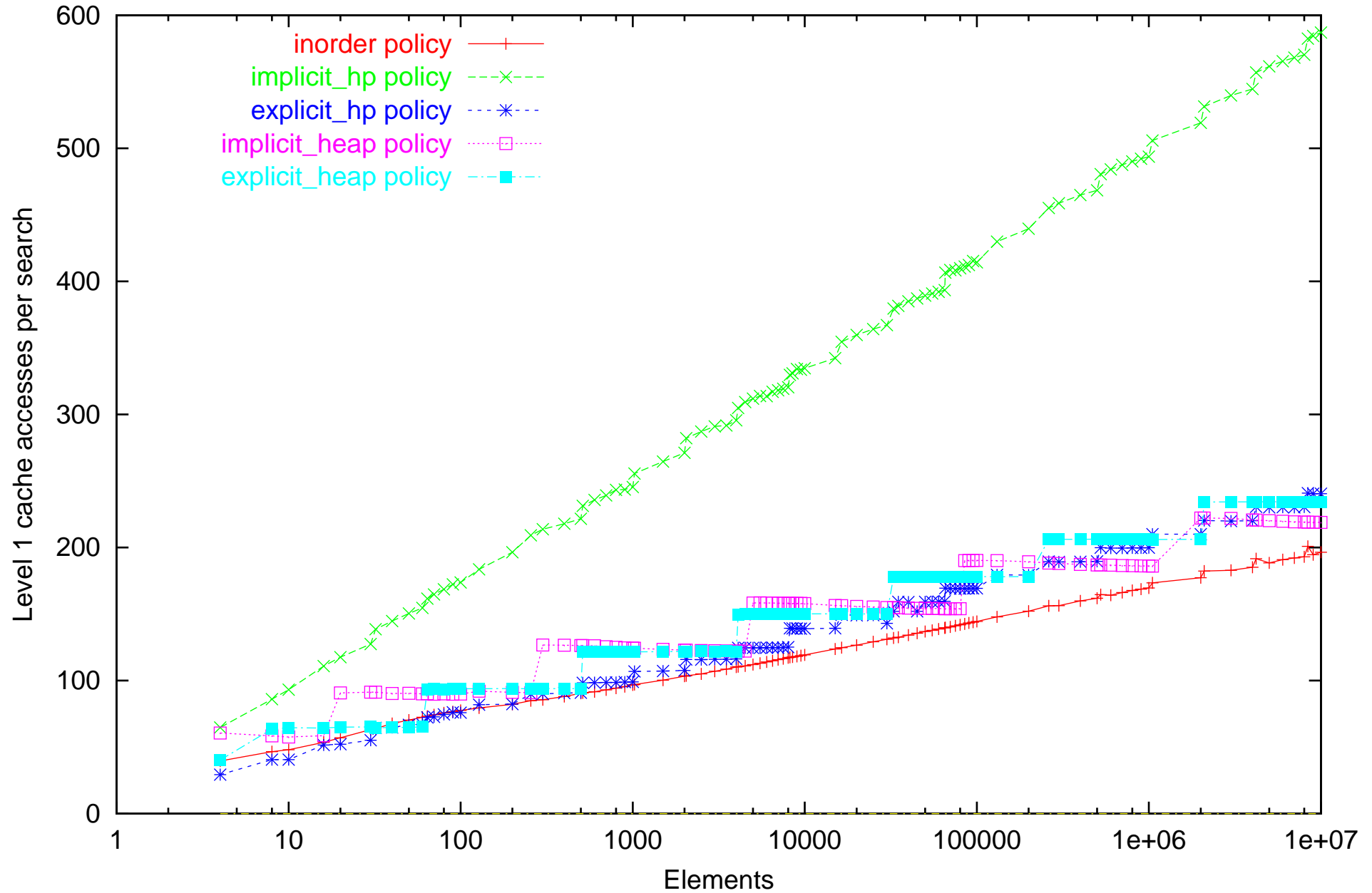
Level 1 cache accesses of static search on Athlon computer. Dataset: successfull_increasing
