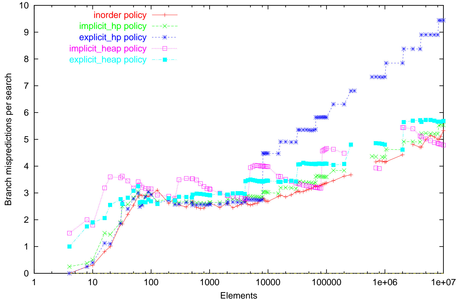
PAPI event count of static search on Athlon computer. Dataset: successfull_increasing
