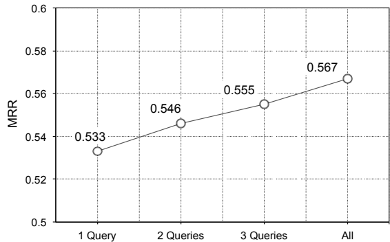
Figure 6: Variation of HRED performance with respect to the number of previous queries considered. The evolution is computed on long sessions.
