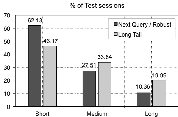
Figure 4: Proportion (%) of short (2 queries), medium (3 or 4 queries) and long (at least 5 queries) sessions in our test scenarios.
